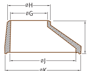
CROSS SECTION
